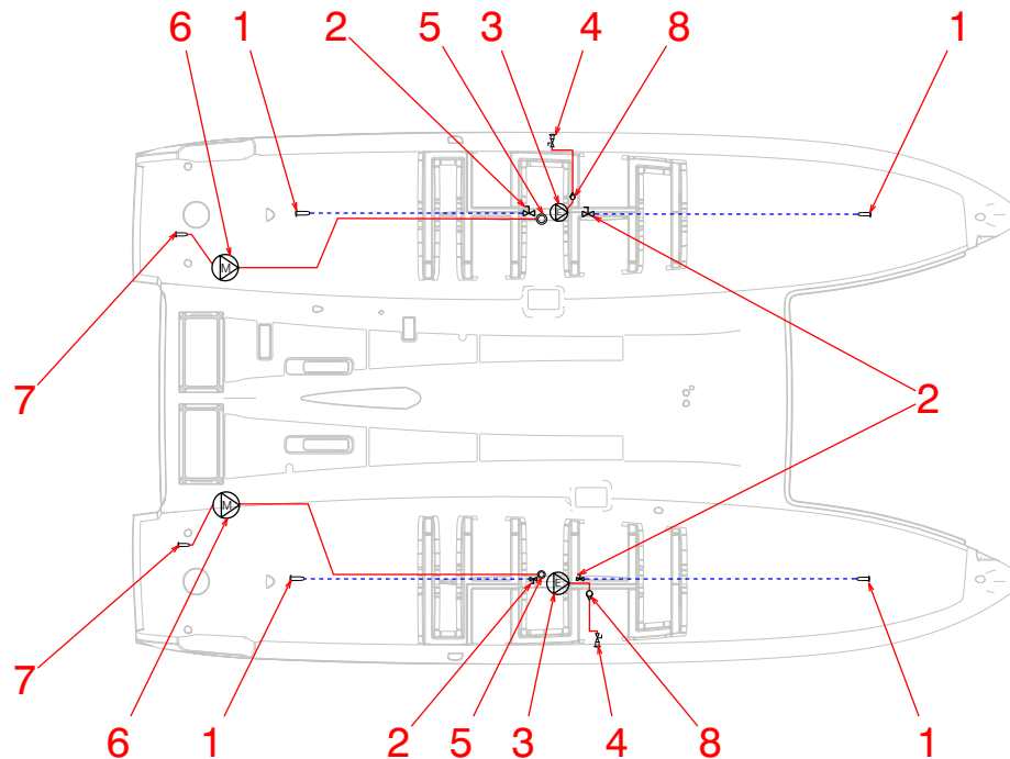
Diagram of Layout – Drying out the bilge
