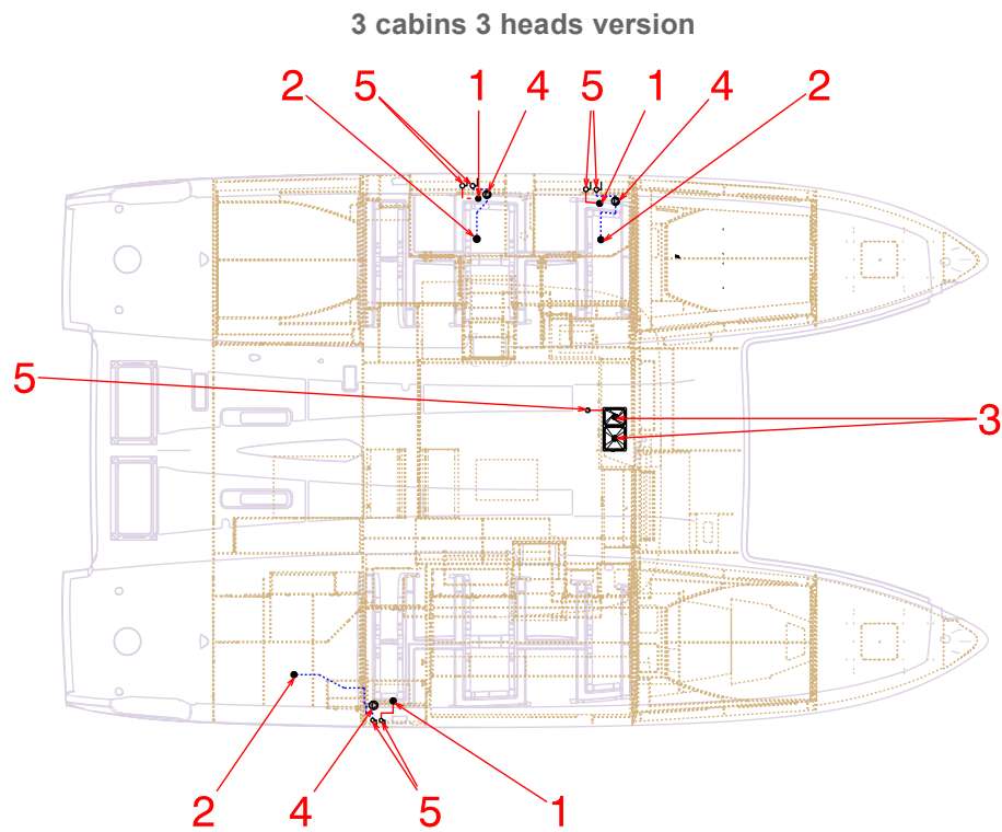
Diagram of waste water circuit installation
