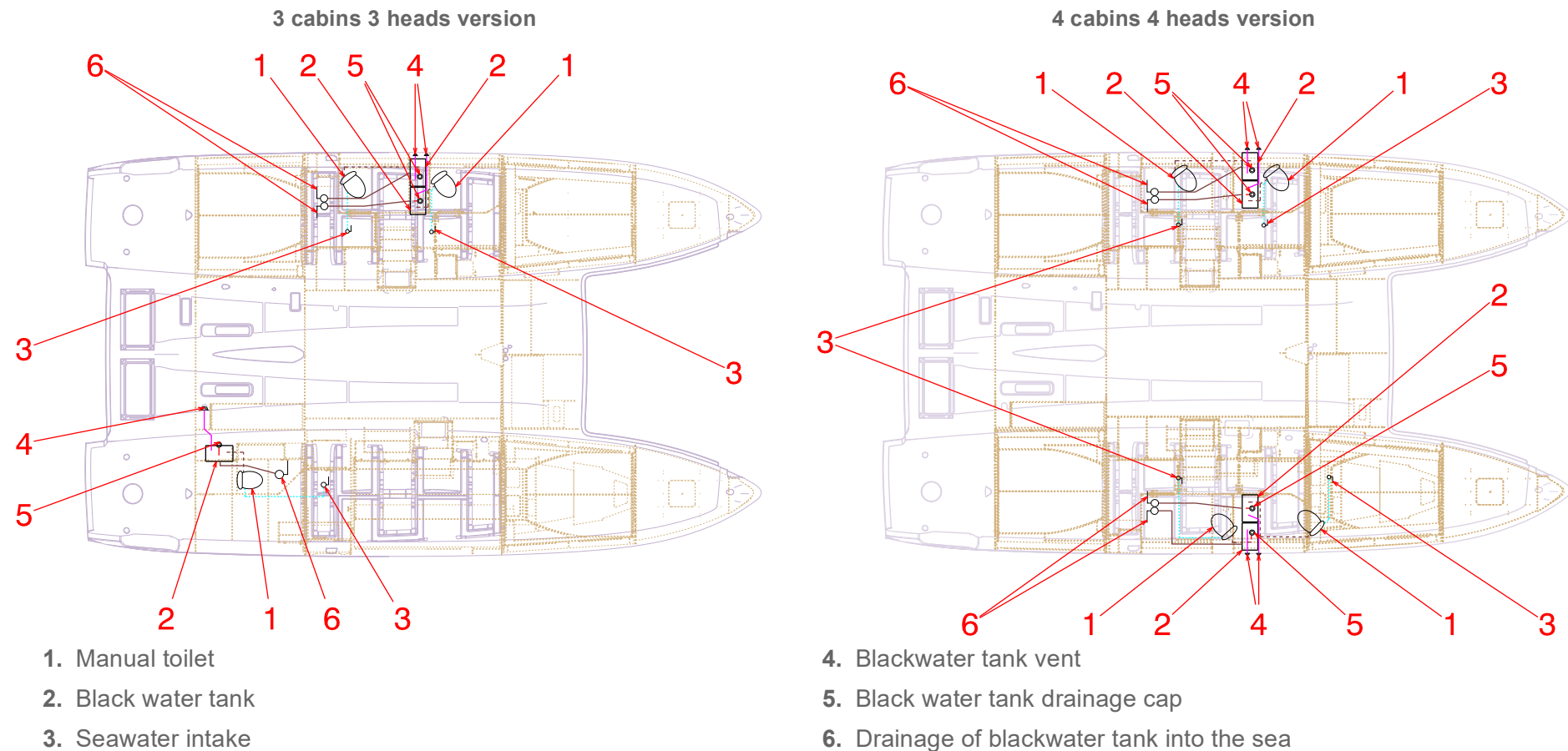
Diagram of blackwater system
